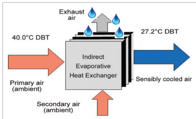
Figure 2: Indirect evaporative cooling
