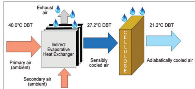
Figure 3: Indirect-direct evaporative cooling
